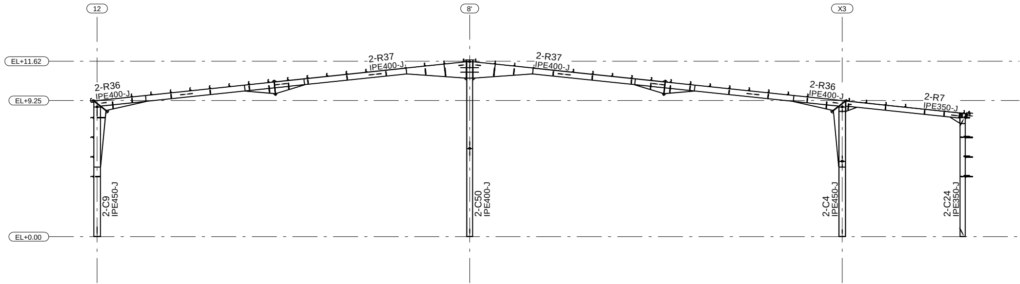
SECTION GRID J
