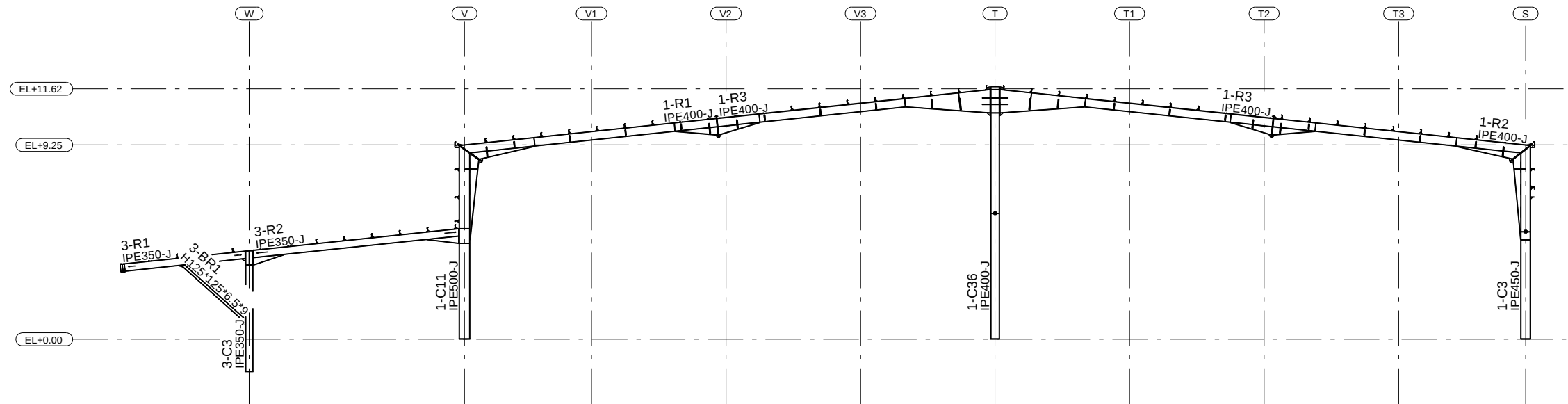
SECTION GRID 2
