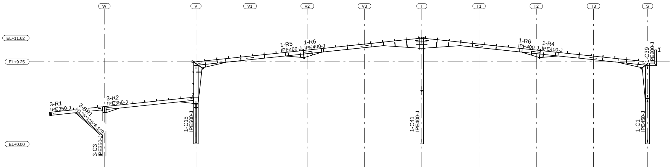
SECTION GRID 10
