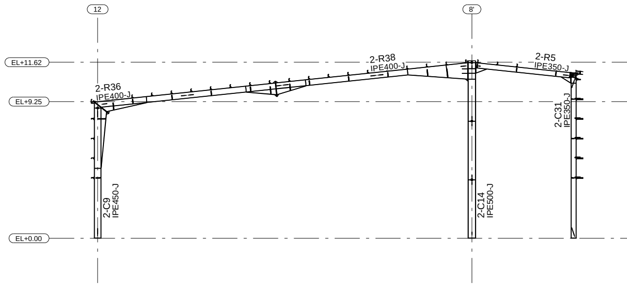
SECTION GRID C
