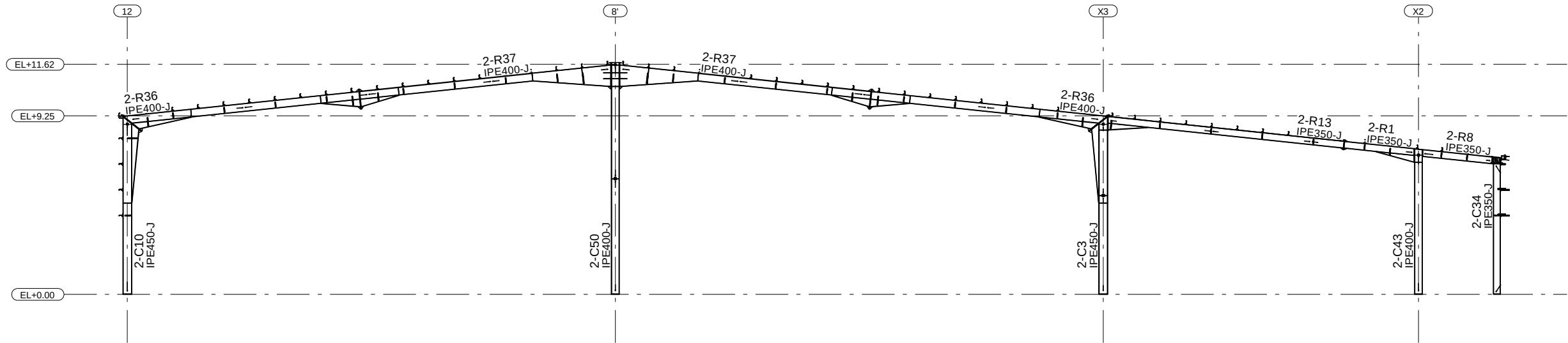
SECTION GRID M
