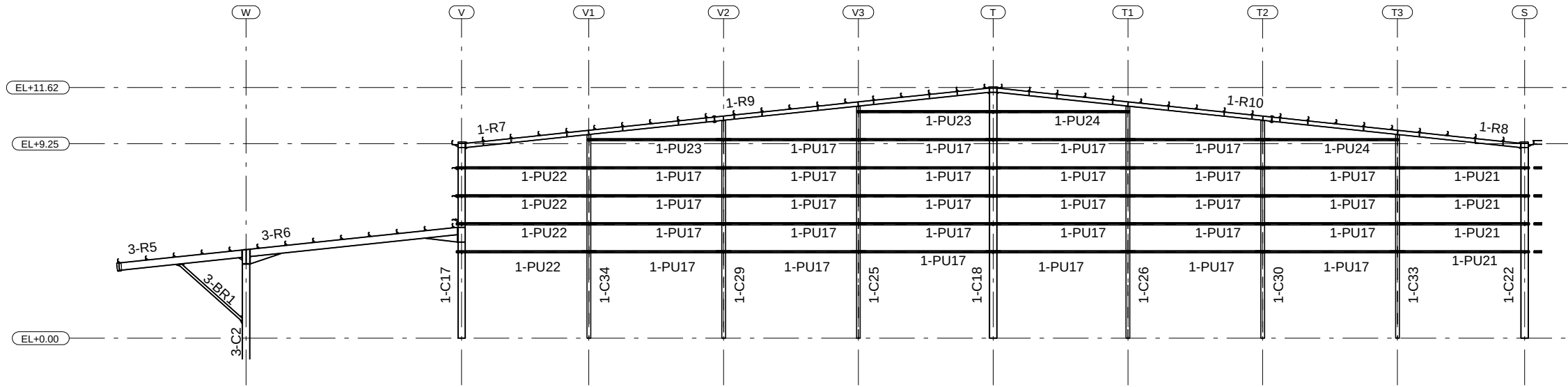
SECTION GRID 12
