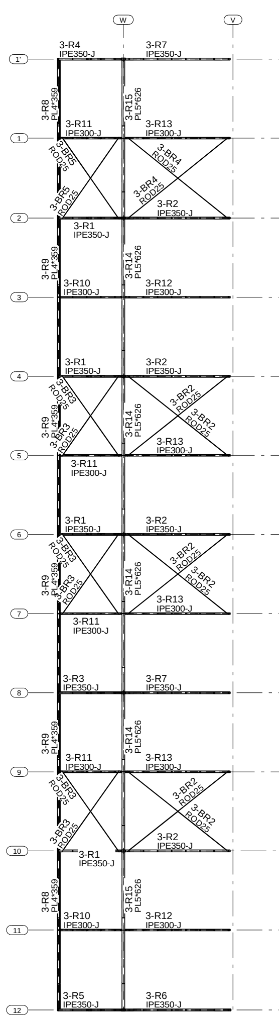
ROOF PLAN WITHOUT PURLIN
