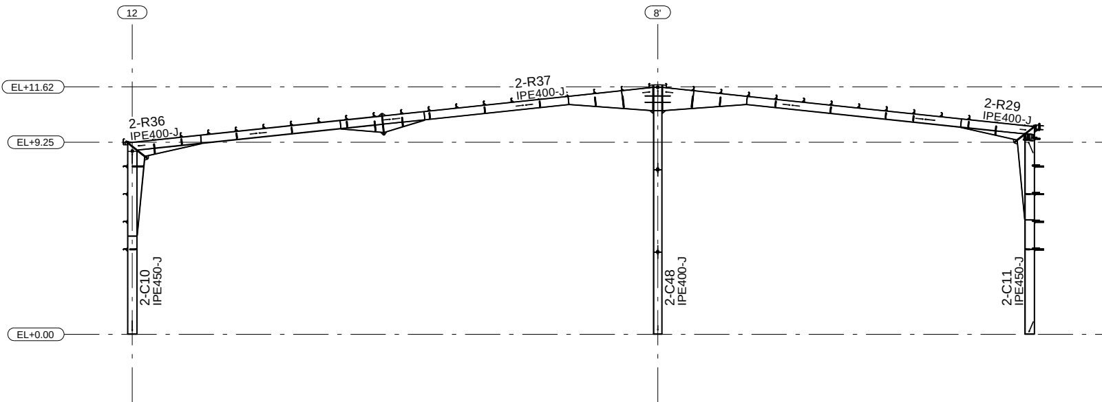
SECTION GRID F
