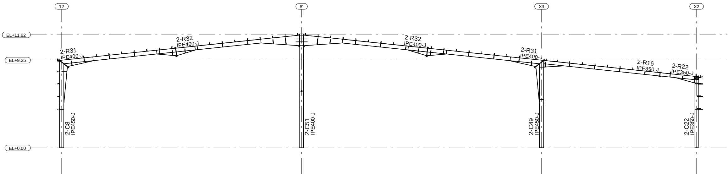
SECTION GRID L
