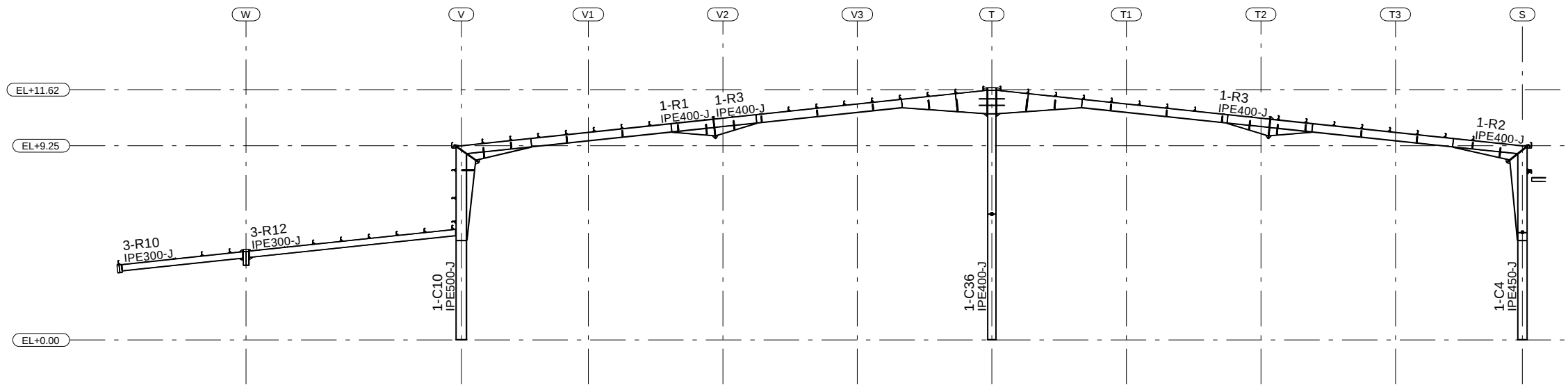
SECTION GRID 3
