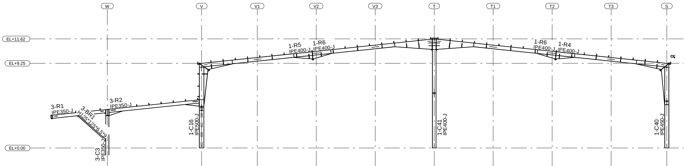
SECTION GRID 6
